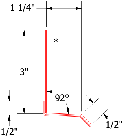
MCA661 - Base Trim
