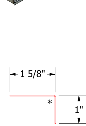
MCA680 - Angle Trim
