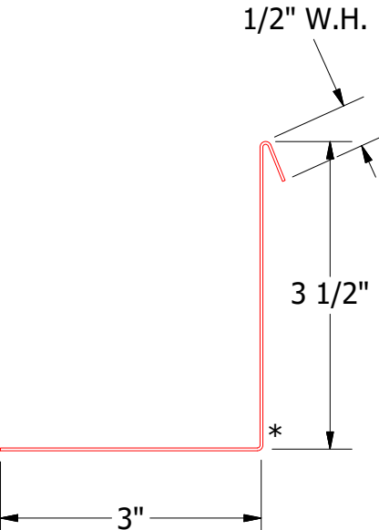
MCA683 - Angle Trim With Return
