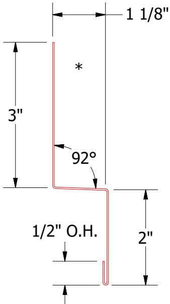
MCA550 - Head Trim
