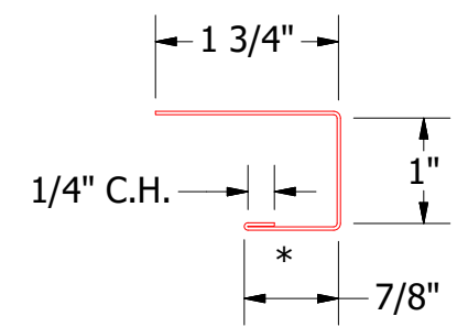
MCA118 - J Channel
