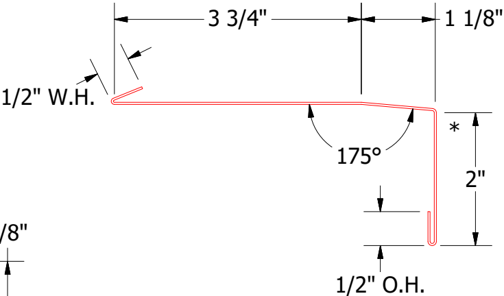
MCA670 - Window Sill Trim
