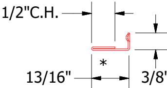
UNS078 - Snap J Cover
