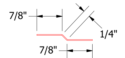
HLA975-Joggle Cleat
