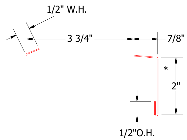
HCA670 - Window Sill Trim
