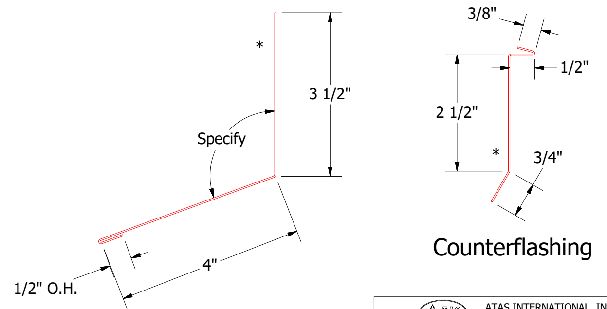
HCA500 - Headwall Trim
