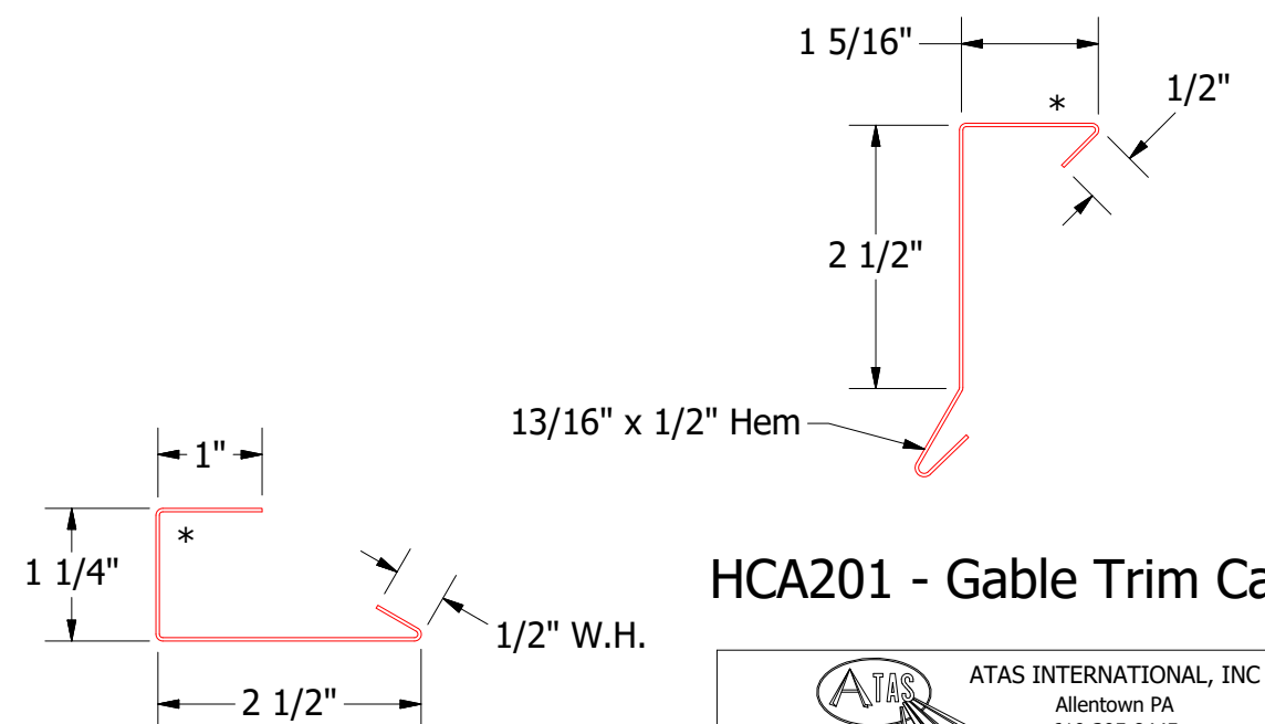
HCA200 - Channel Trim
