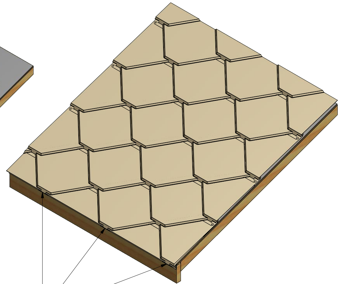
Fold CastleTop Tabs around Drip Edge Trim
