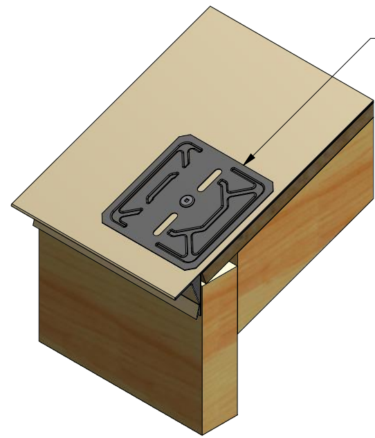
Bearing Plate used at Eave in High Wind Applications
