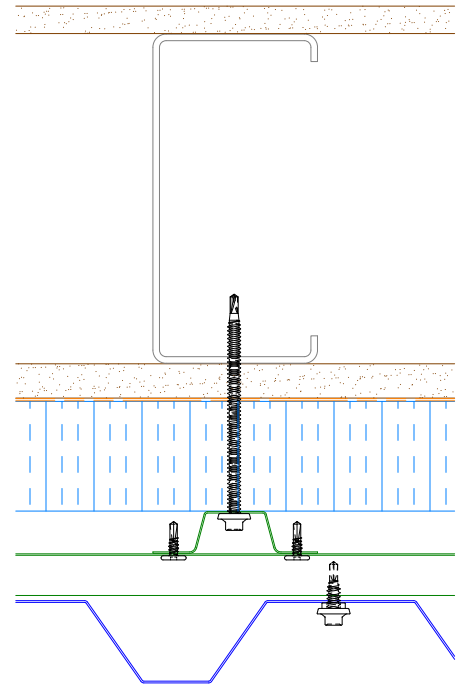
Alternate Subgirt Orientation
