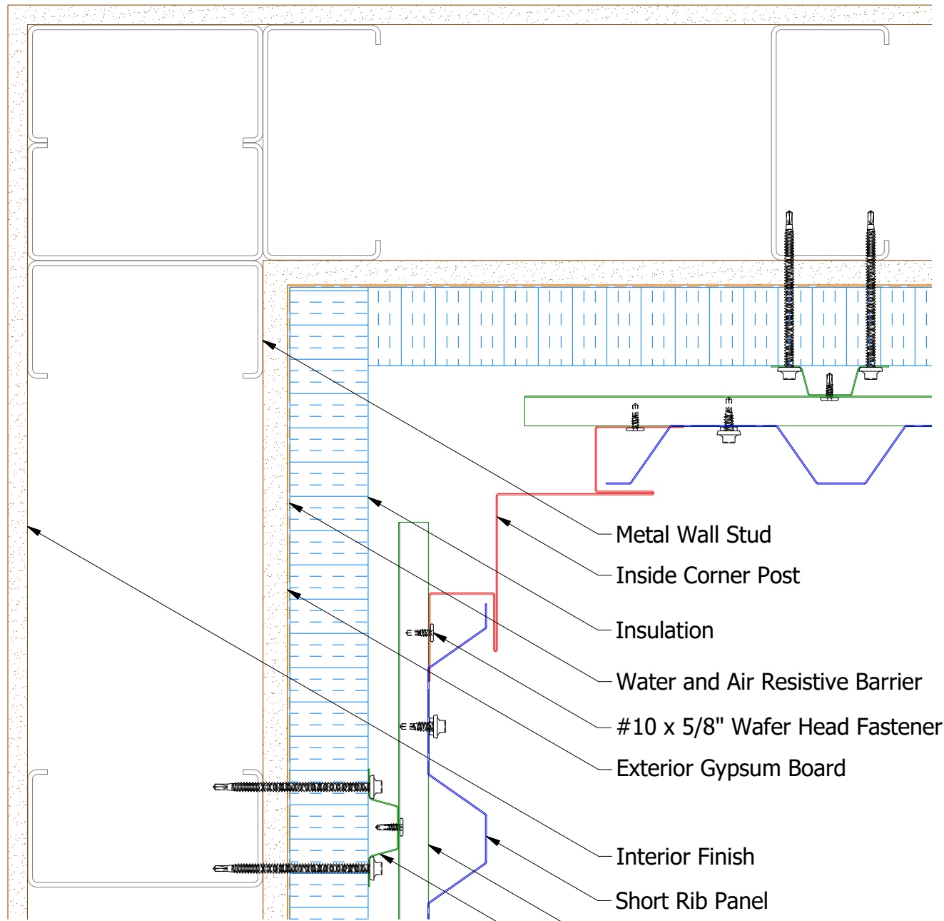
Alternate Subgirt Orientation
