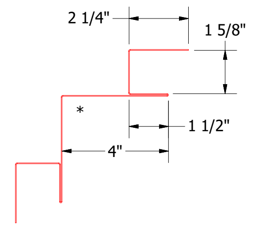
BWA601-Inside Corner Post
