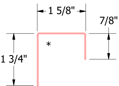
BWA270-J Closure
