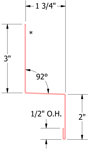
BWA550-Head Trim
