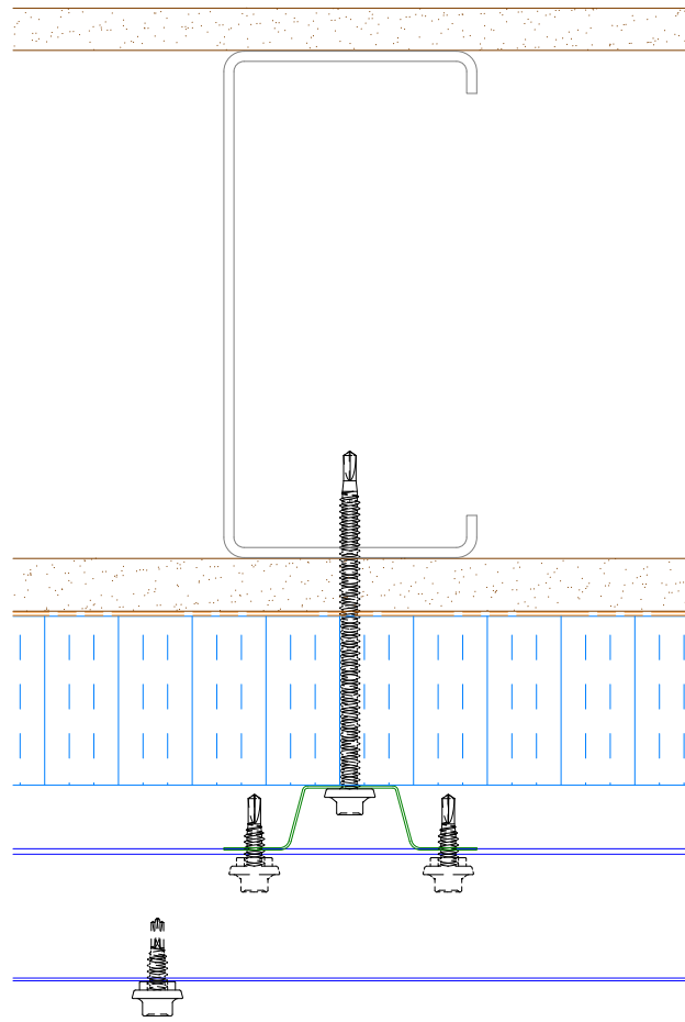
Alternative Subgirt Orientation (NTS)
