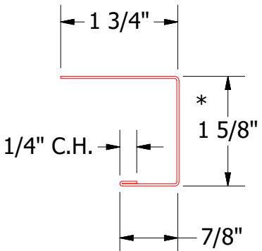
BWA158-J Channel
