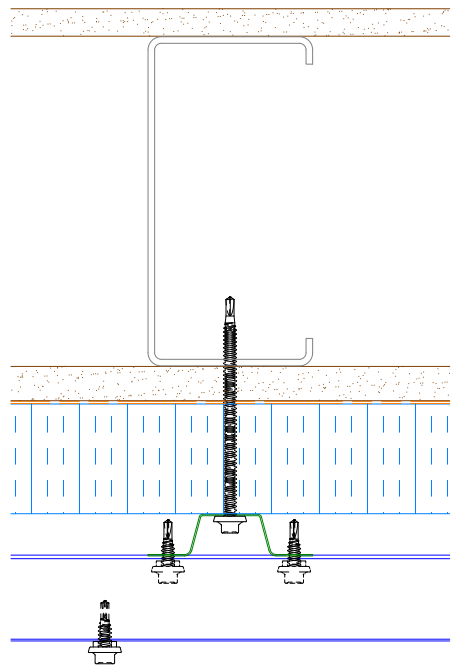
Alternate Subgirt Orientation
