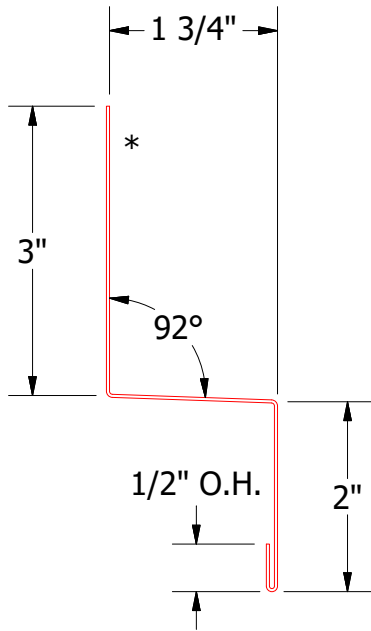
BWA550-Head Trim
