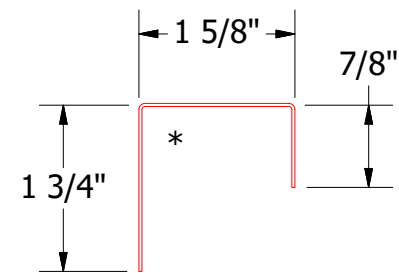
BWA270-J Closure
