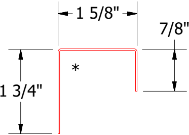
BWA270-J Closure
