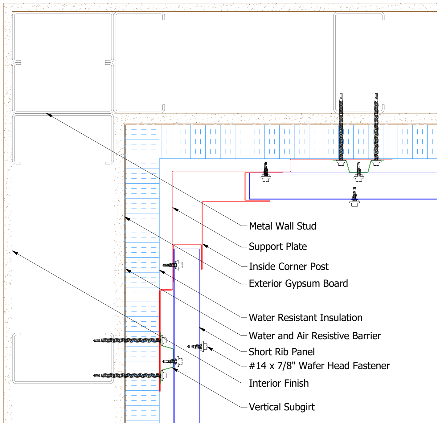
Alternate Subgirt Orientation
