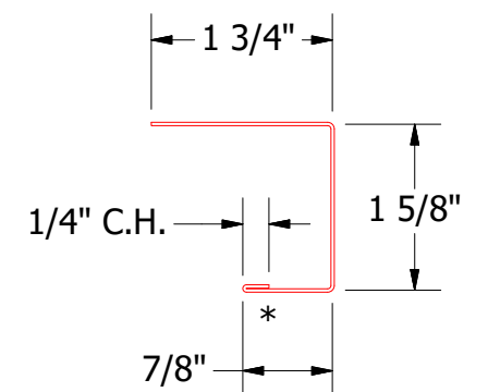
BWA158-J Channel
