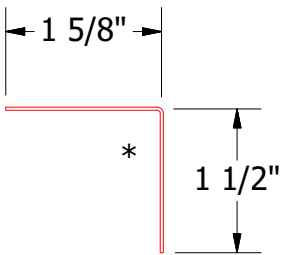
BWA680-Angle Trim
