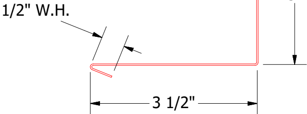
BWA683-Angle Trim with Return (Field Fabricated from Color Matched Flat Stock)
