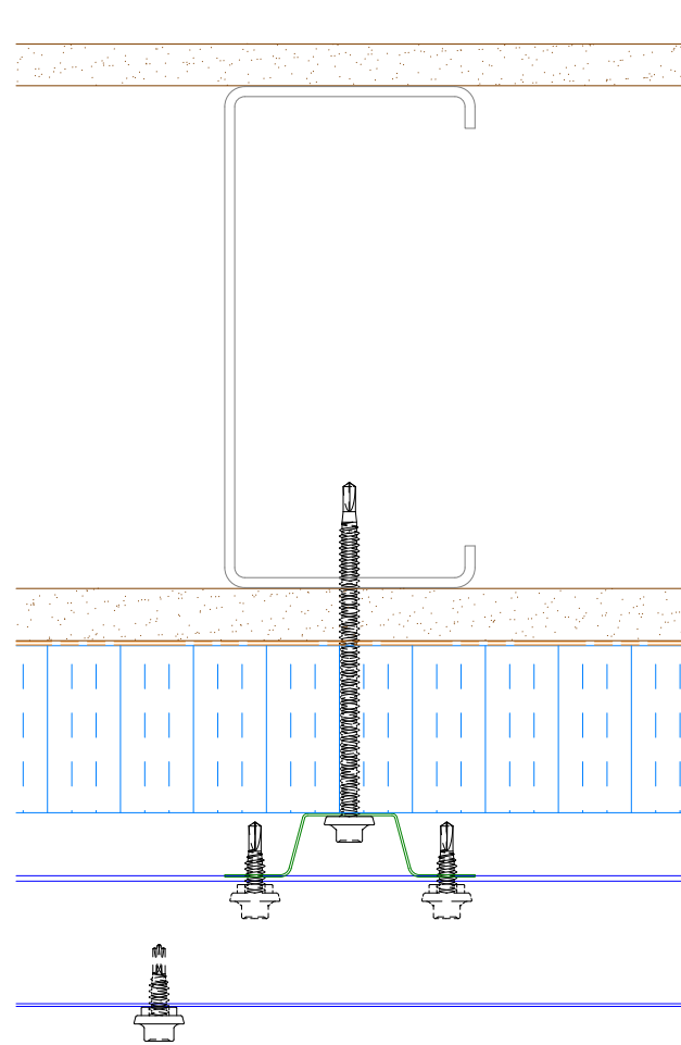
Alternative Subgirt Orientation (NTS)
