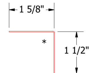
BWA680-Angle Trim
