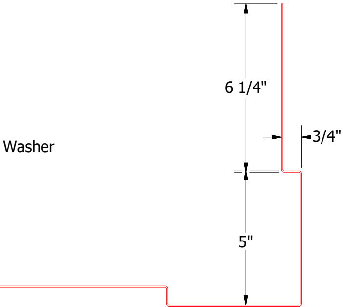
Support Plate
