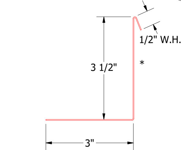
BWA683-Angle with Return
