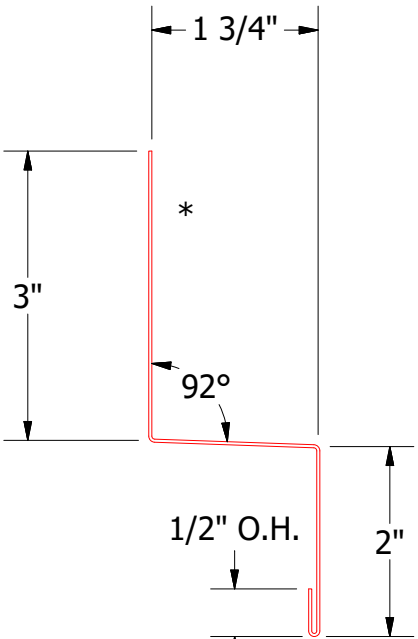
BWA550-Head Trim
