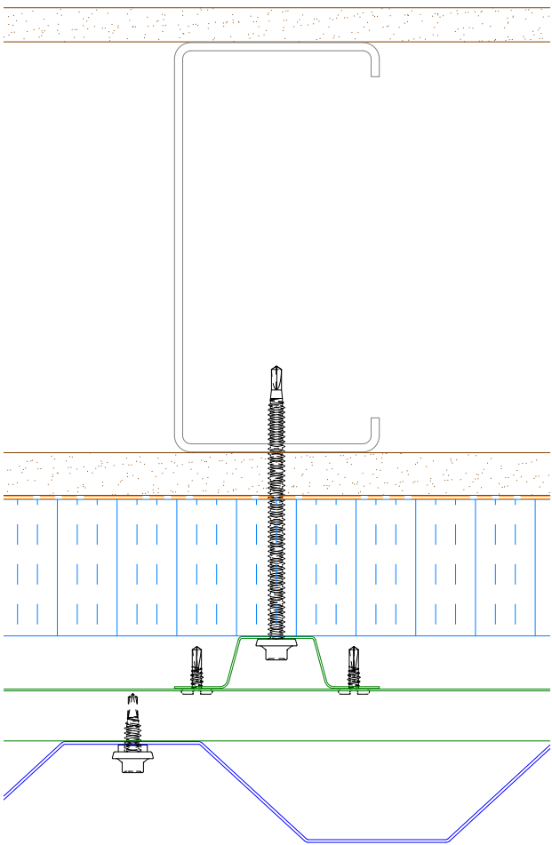
Alternate Subgirt Orientation
