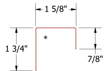
BWA270-J Closure
