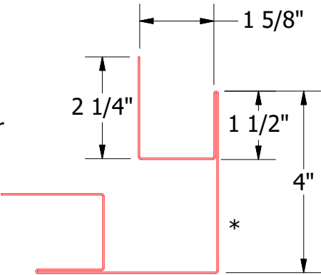
BWA602-Outside Corner Post
