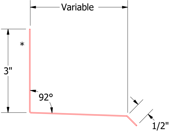
Flashing
