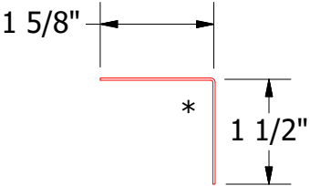
BWR680-Angle Trim
