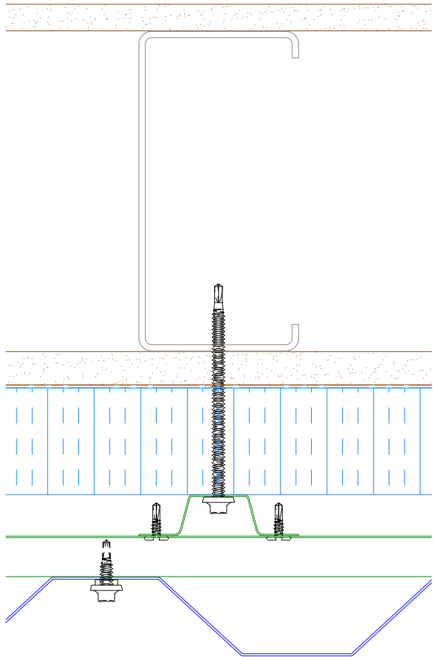
Alternate Subgirt Orientation
