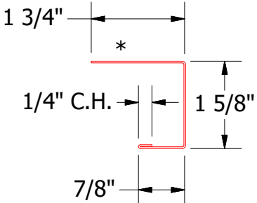
BWR158-J Channel
