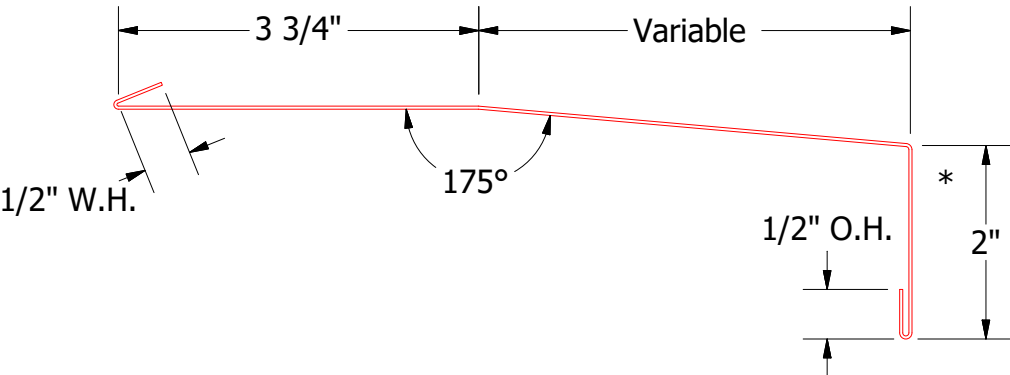
BWA670-Window Sill Trim
