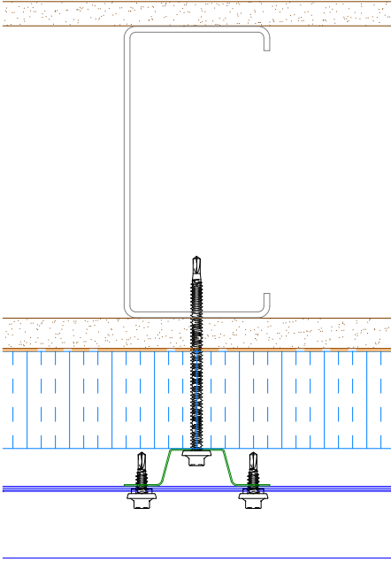
Alternative Subgirt Orientation
