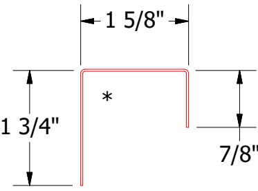
BWA270-J Closure
