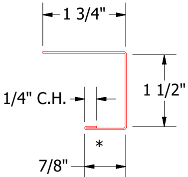
BWA158-J Channel
