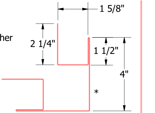
BWA602-Outside Corner Post
