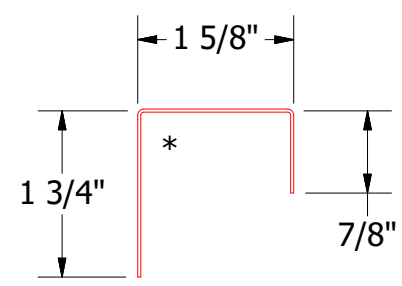
BWA270-J Closure
