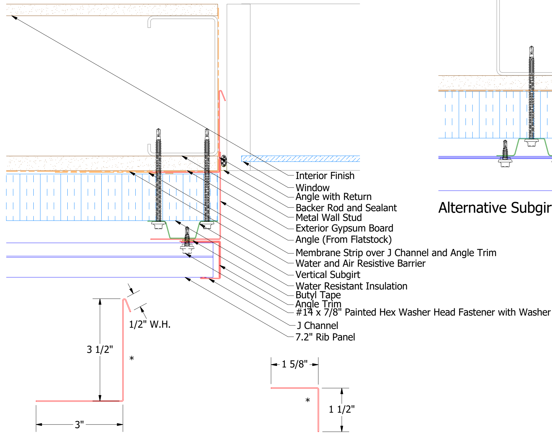
BWA683-Angle with Return
