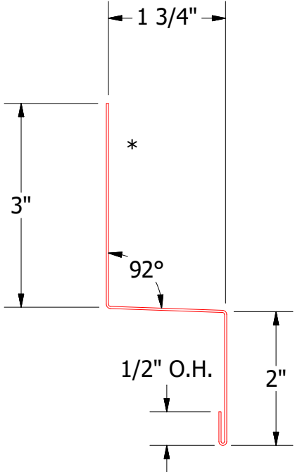
BWA550-Head Trim
