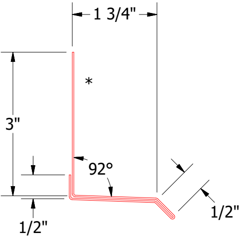
BWA661-Base Trim
