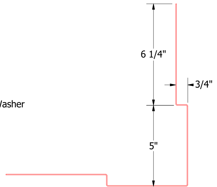
Support Plate
