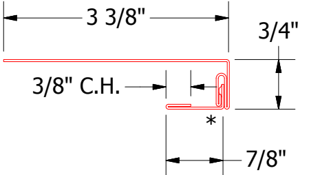
BGA309 - Snap J Channel
