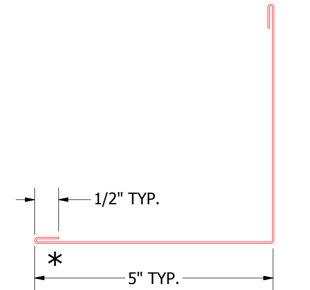
MDA610-Outside Corner Cap
