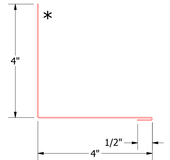
MDA410-Sidewall Trim
