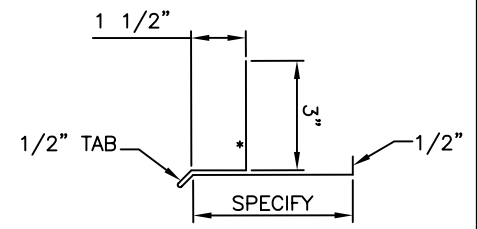
MPA661 CLOSED SILL TRIM
