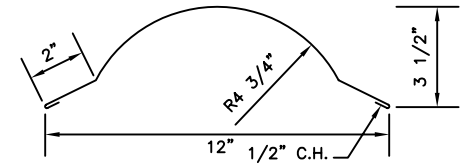
SCA370 RIDGE CAP
