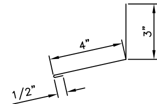
HSA500 HEADWALL TRIM
