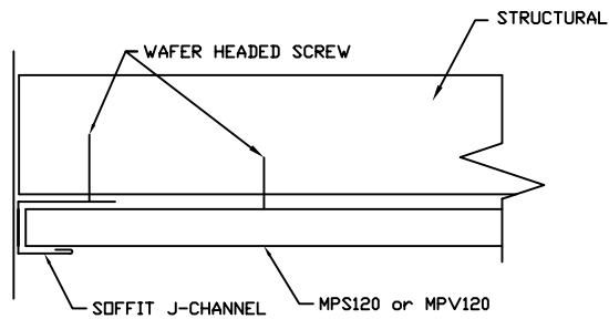
J-CHANNEL DETAIL SCALE: NONE
