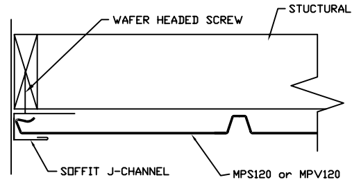
J-CHANNEL DETAIL SCALE: NONE
