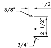
COUNTERFLASHING - SCA980T3?? 12'-0" Long each.
