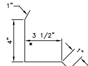
1/2" C.H. SIDEWALL TRIM - SCA412T3?? 12'-0" Long
