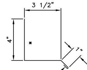
1/2" C.H. SIDEWALL TRIM - SCA410T3?? 12'-0" Long
