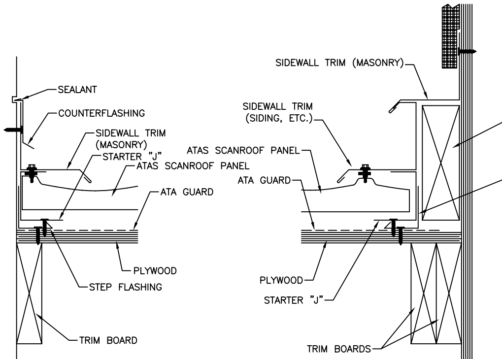
STEP FLASHING - SCA420T3?? 1'-6" Long
