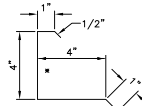
1/2" C.H. SIDEWALL TRIM - SCA411T3?? 12'-0" Long
