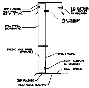
BWK360 Panel Vertical Application Cap and Sill Detail
