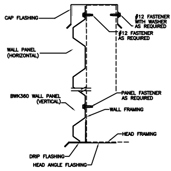
BWK360 Panel Horizontally Application Cap and Sill Detail
