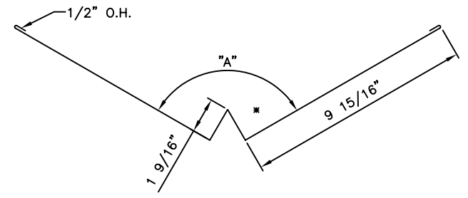
PCA800 VALLEY PAN Angle "A" = Customer to specify or furnish slope(s) involved.
