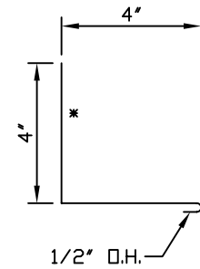
②③ - MDA410 SIDEWALL TRIM
