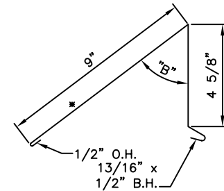
SHED RIDGE CAP PCA346 - Roof Slopes 9/12+ to 12/12 Ridge splice to match ridge cap @ 6' long each; PCA347
