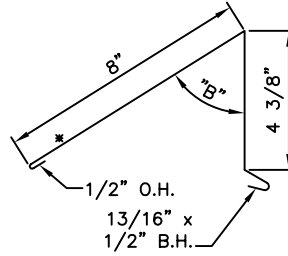
SHED RIDGE CAP PCA344 - Roof Slopes 6/12+ to 9/12 Ridge splice to match ridge cap @ 6' long each; PCA345
