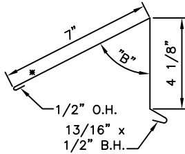
SHED RIDGE CAP PCA342 - Roof Slopes 3/12+ to 6/12 Ridge splice to match ridge cap @ 6' long each; PCA343
