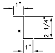
PCA912 - 'Z' CLOSURE
