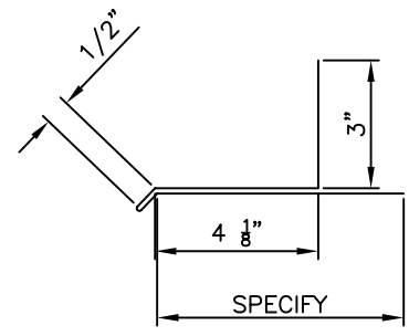
HEAD TRIM
