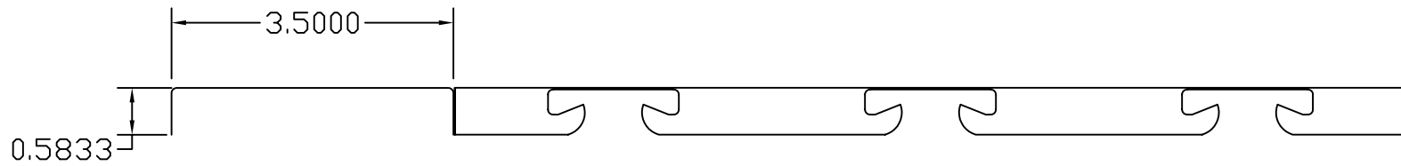
Suspended Box Carrier
