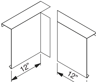
INSIDE CORNER
