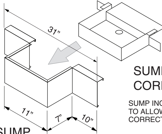
SUMP FACE
