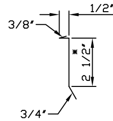
(22) - MDA980 COUNTERFLASHING
