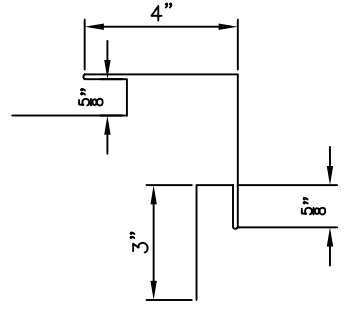
OUTSIDE CORNER TRIM
