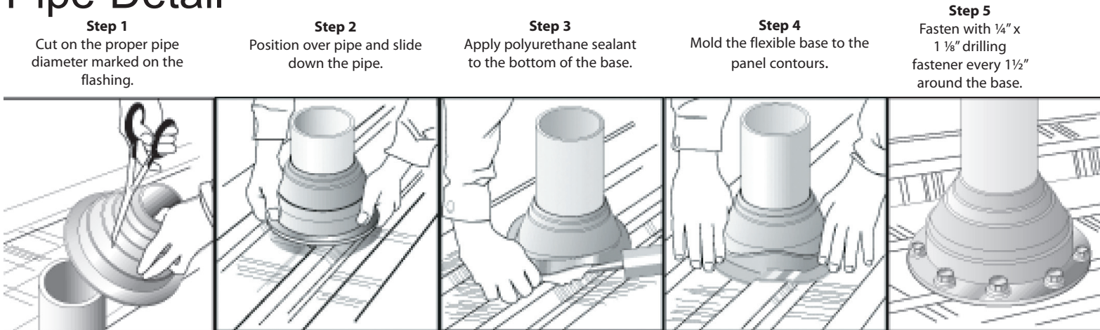
Pipe drawings provided by Triangle Fasteners
