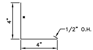
PCA415 STEP FLASHING
