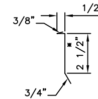
PCA980 COUNTERFLASHING
