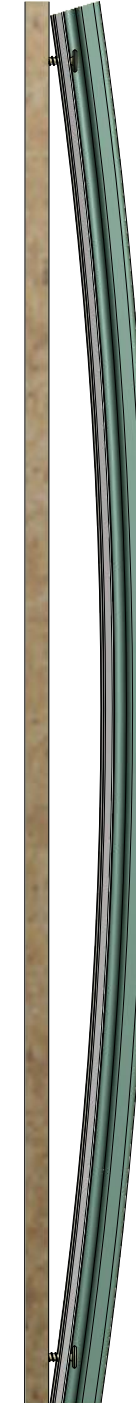
Incorrect Install (Fastening from the Outer Edge to the Middle Will Cause Bowing in the Panel)
