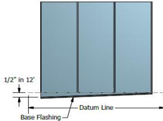
Base Flashing Alignment
