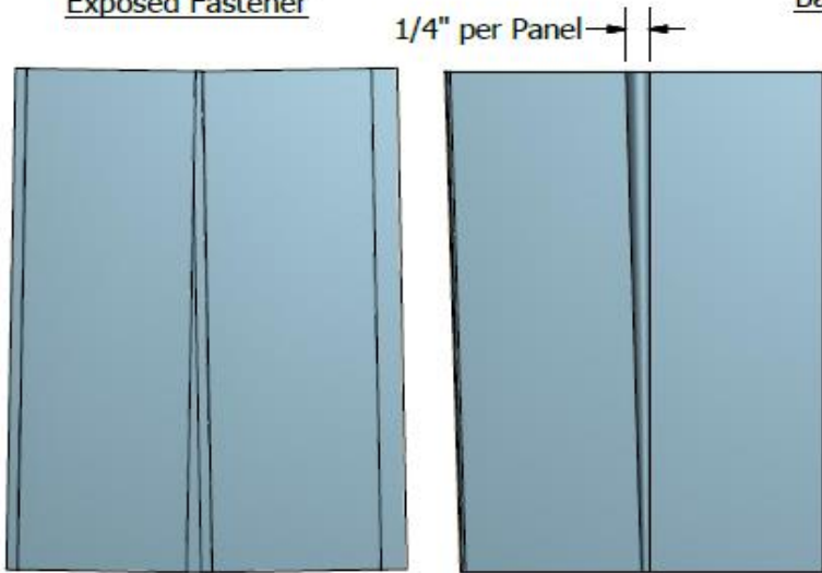
Standing Rib Panel Coverage Variation
